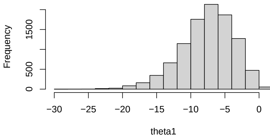
Histogram of theta1
