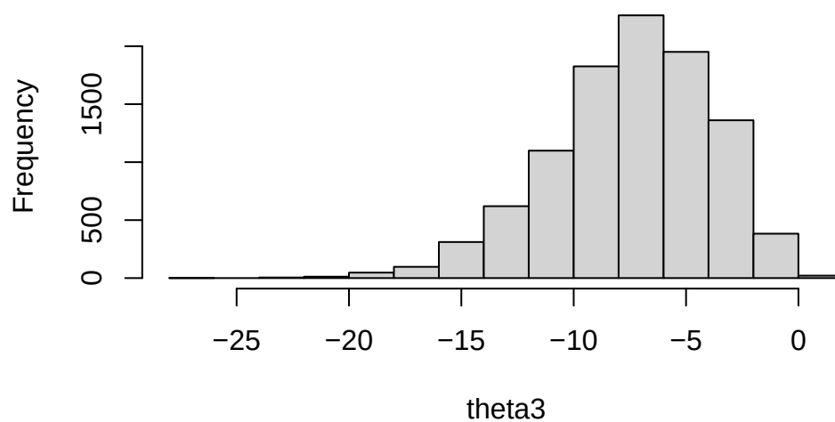
Histogram of theta3
